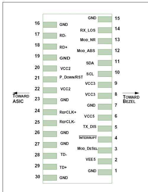
Figure 2.Pin function definitions
