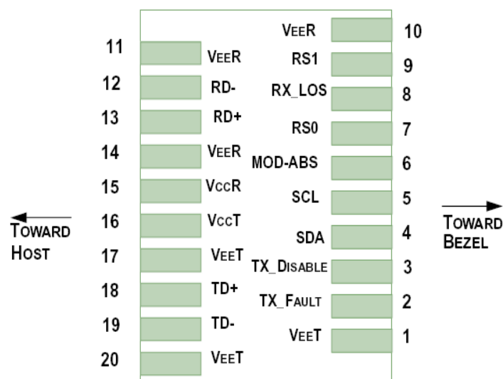
Figure 2.Pin function definitions
