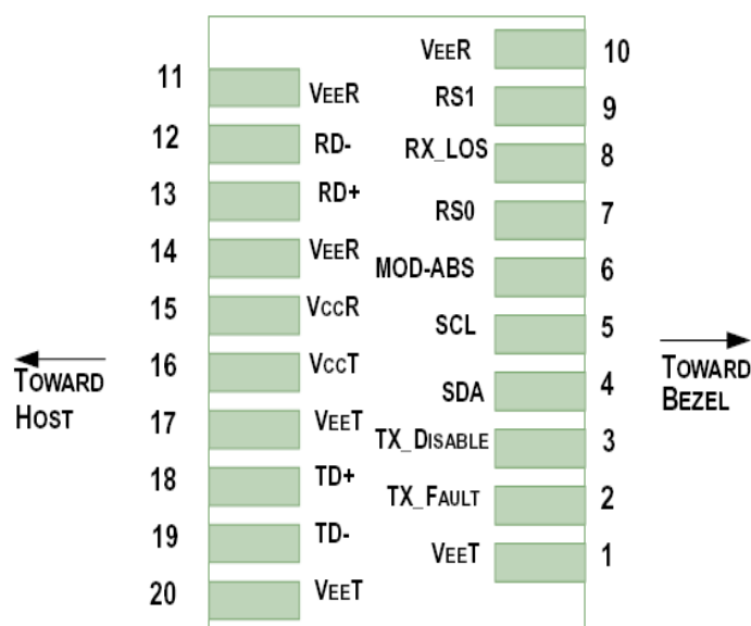
Figure 2.Pin function definitions
